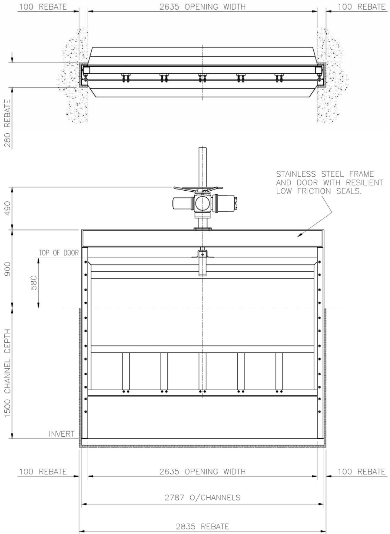
Typical drawing only of a Channel Mounting Type Wedeco Weir Penstock complete with Electric Rotork Actuator and Probe Bracket Grade 304ss Frame and Weir Door.
