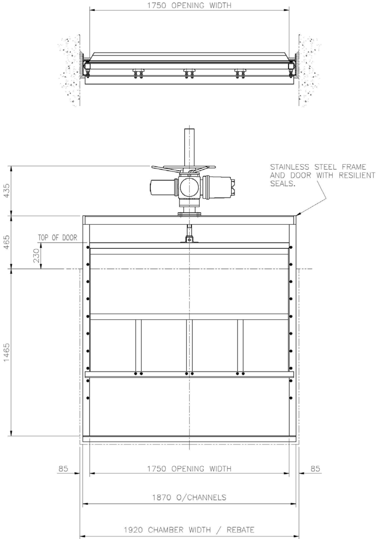
Typical drawing only of a Side Wall Mounting Type Wedeco Weir Penstock complete with Electric Rotork Actuator and Probe Bracket Grade 304ss Frame and Weir Door.
