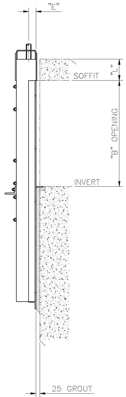
SIDE ELEVATION
