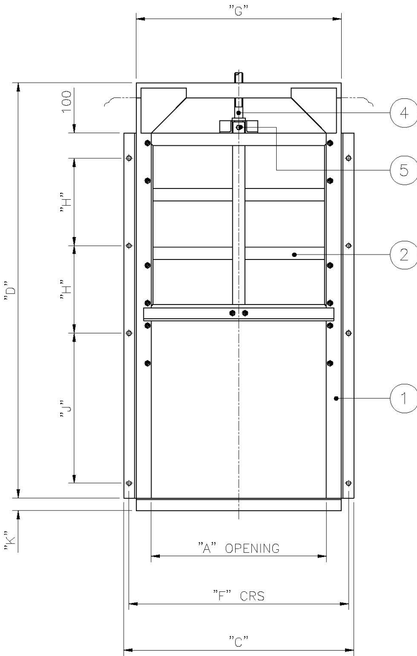
FRONT ELEVATION
